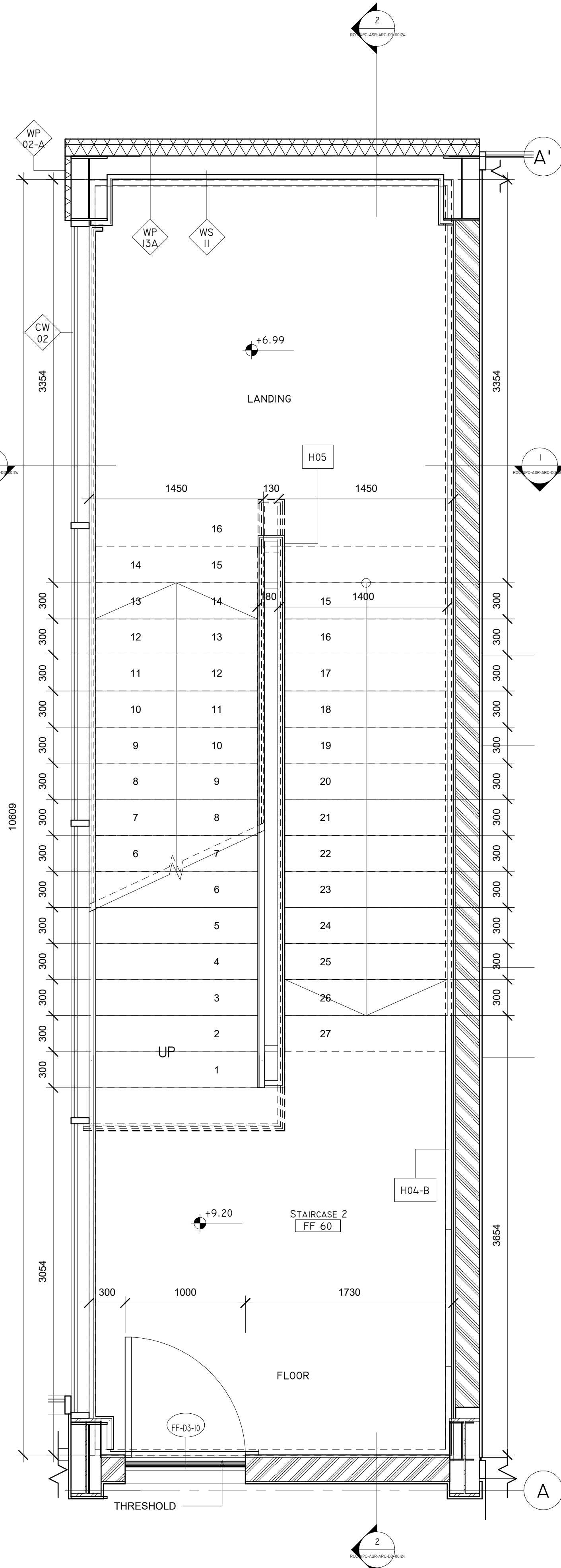
03 FIRST FLOOR PLAN (STAIRCASE -2) 1 : 25
