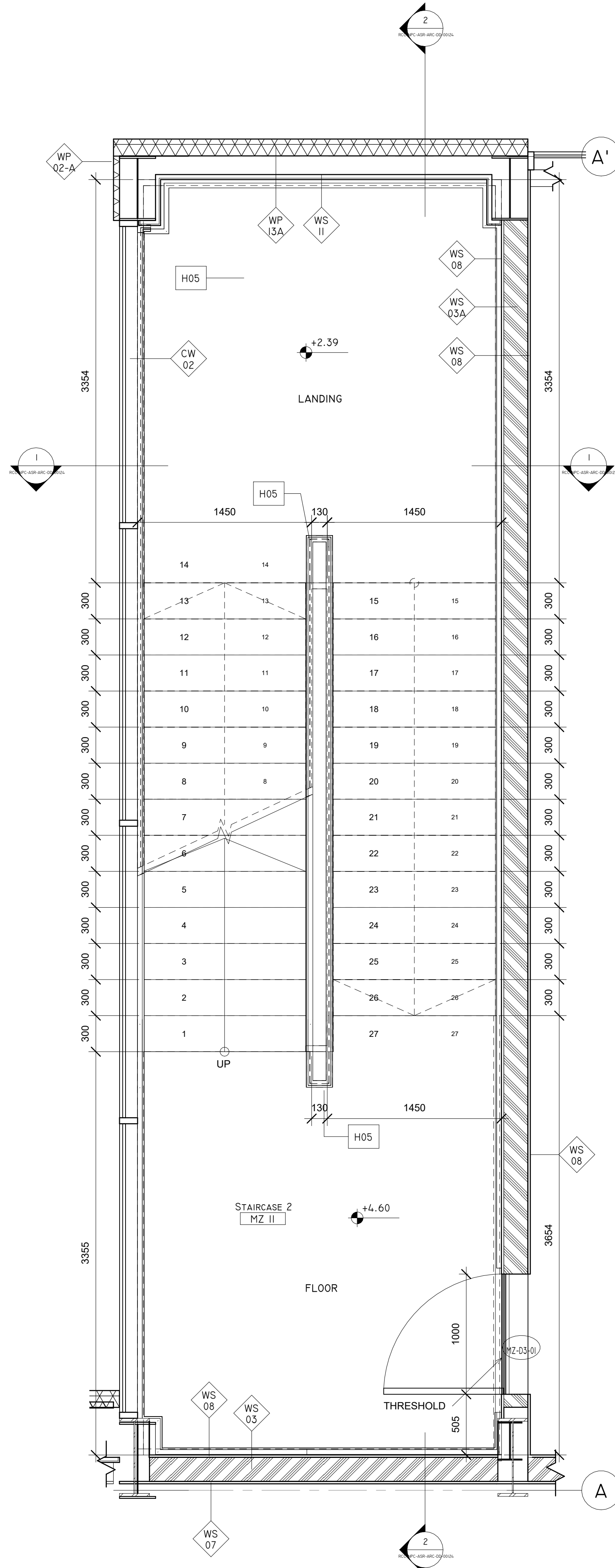
02 MEZZANINE FLOOR PLAN (STAIRCASE -2) 1 : 25
