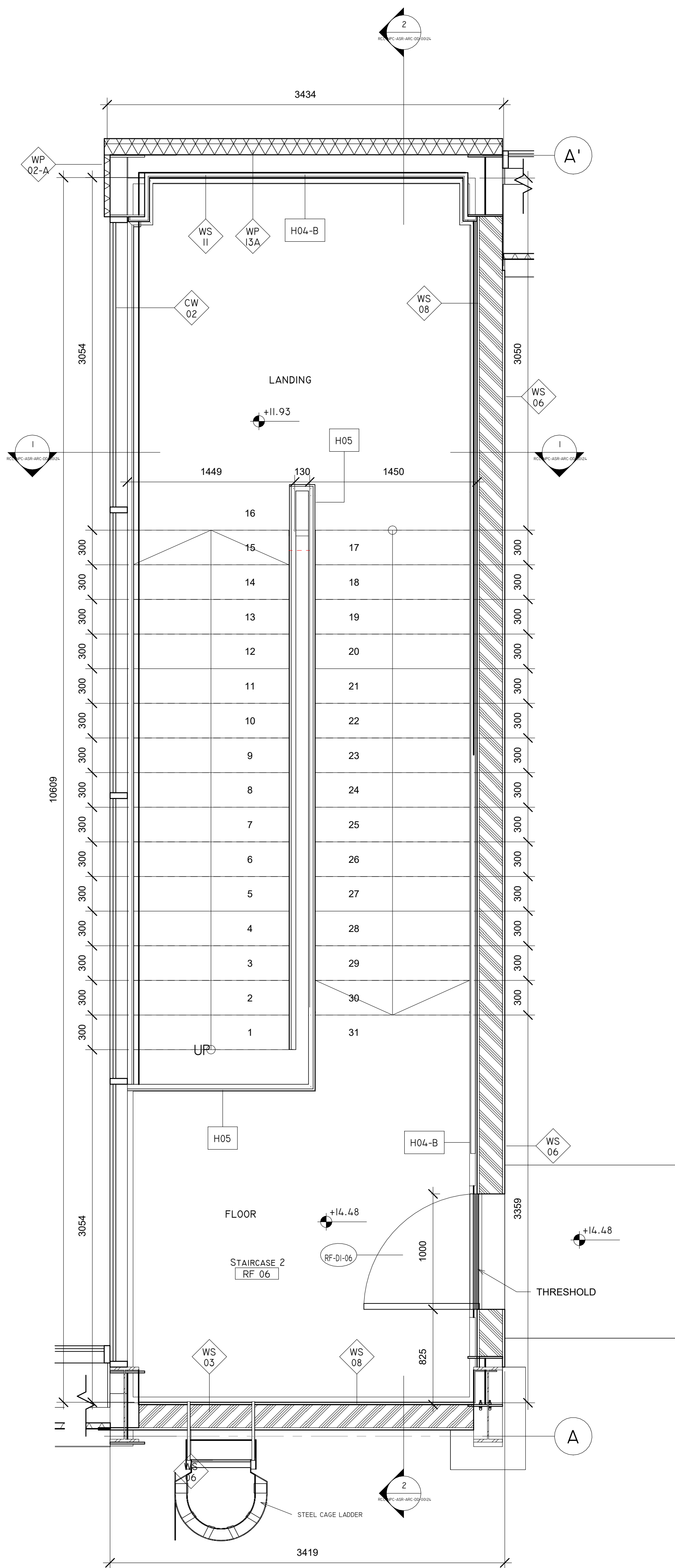
04 ROOF FLOOR PLAN (STAIRCASE -2) 1 : 25
