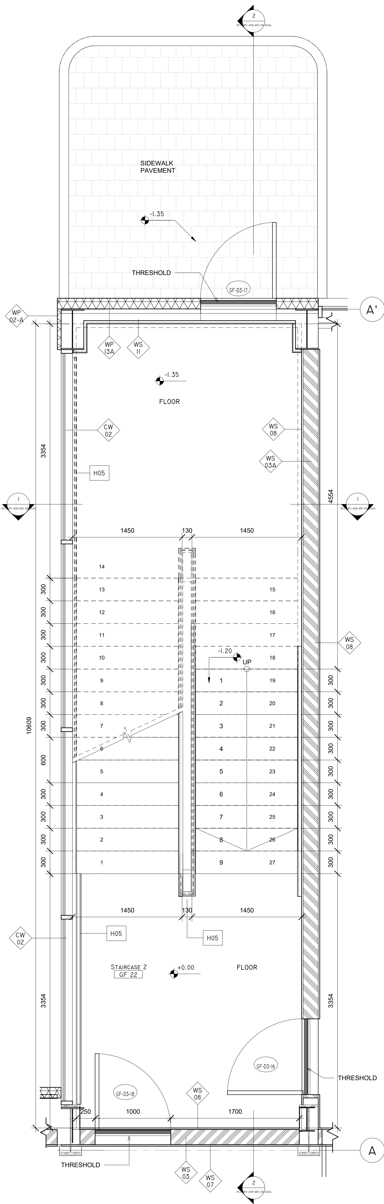
01 GROUND FLOOR PLAN (STAIRCASE -2) 1 : 25
